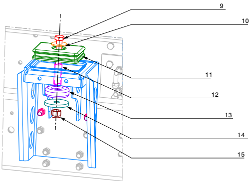
MOUNTING DETAILS FOR B1A09803
