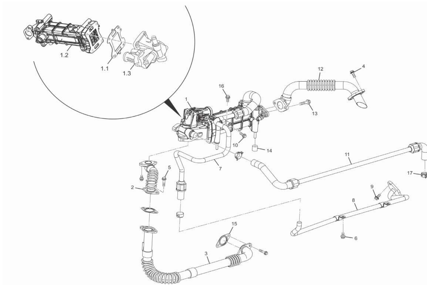
EGR SYSTEM - A2G05000 - HAEGR17
