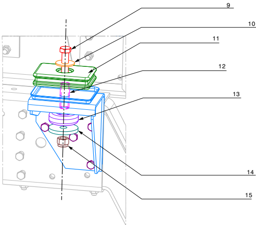
MOUNTING DETAILS FOR B1A09801 & B1A09802
