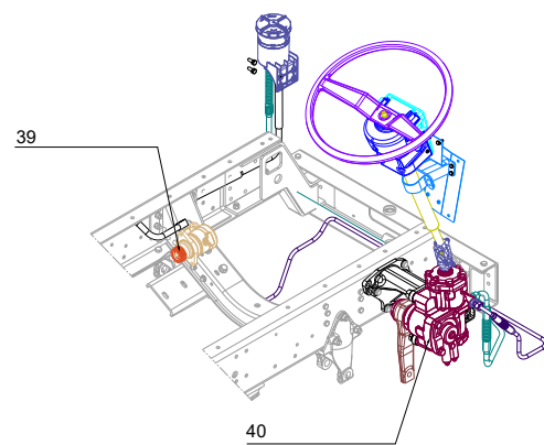
ZF POWER STEERING GEARBOX ASSY
