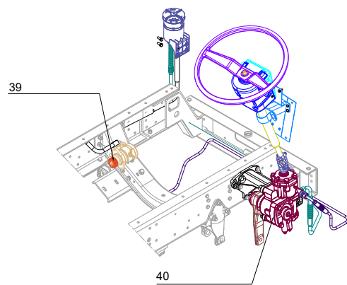
ZF POWER STEERING GEARBOX ASSY
