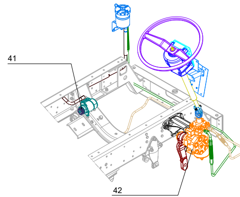
RANE POWER STEERING GEARBOX ASSY
